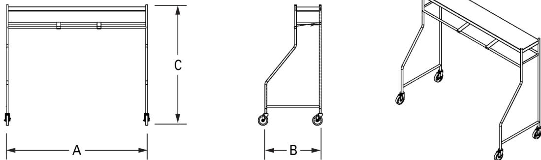
CANTILEVER STYLE 411-1217, 411-1218, 411-1219
